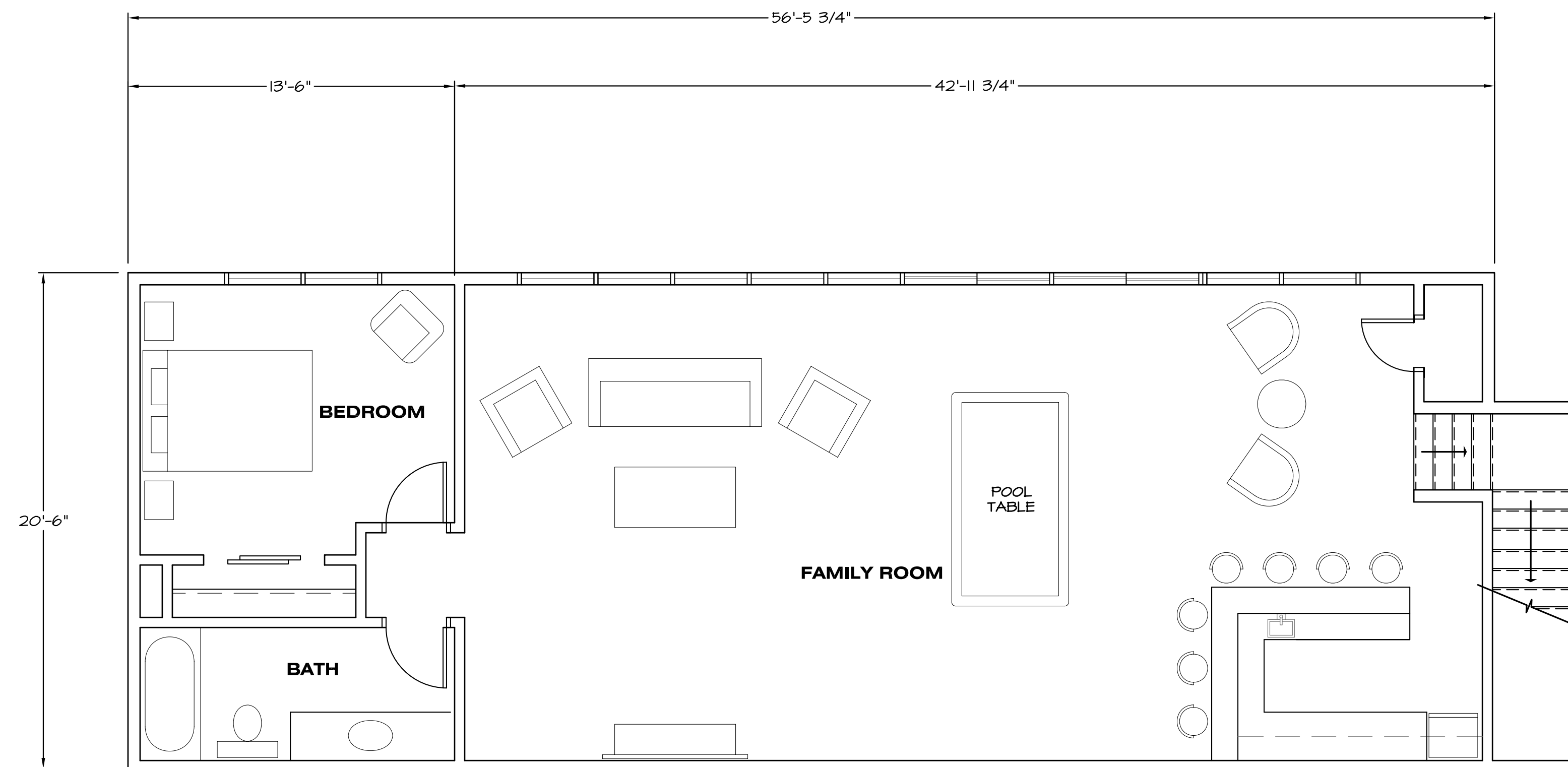
FLOOR PLAN - BASEMENT SCALE: 1/4" = 1'-0"
